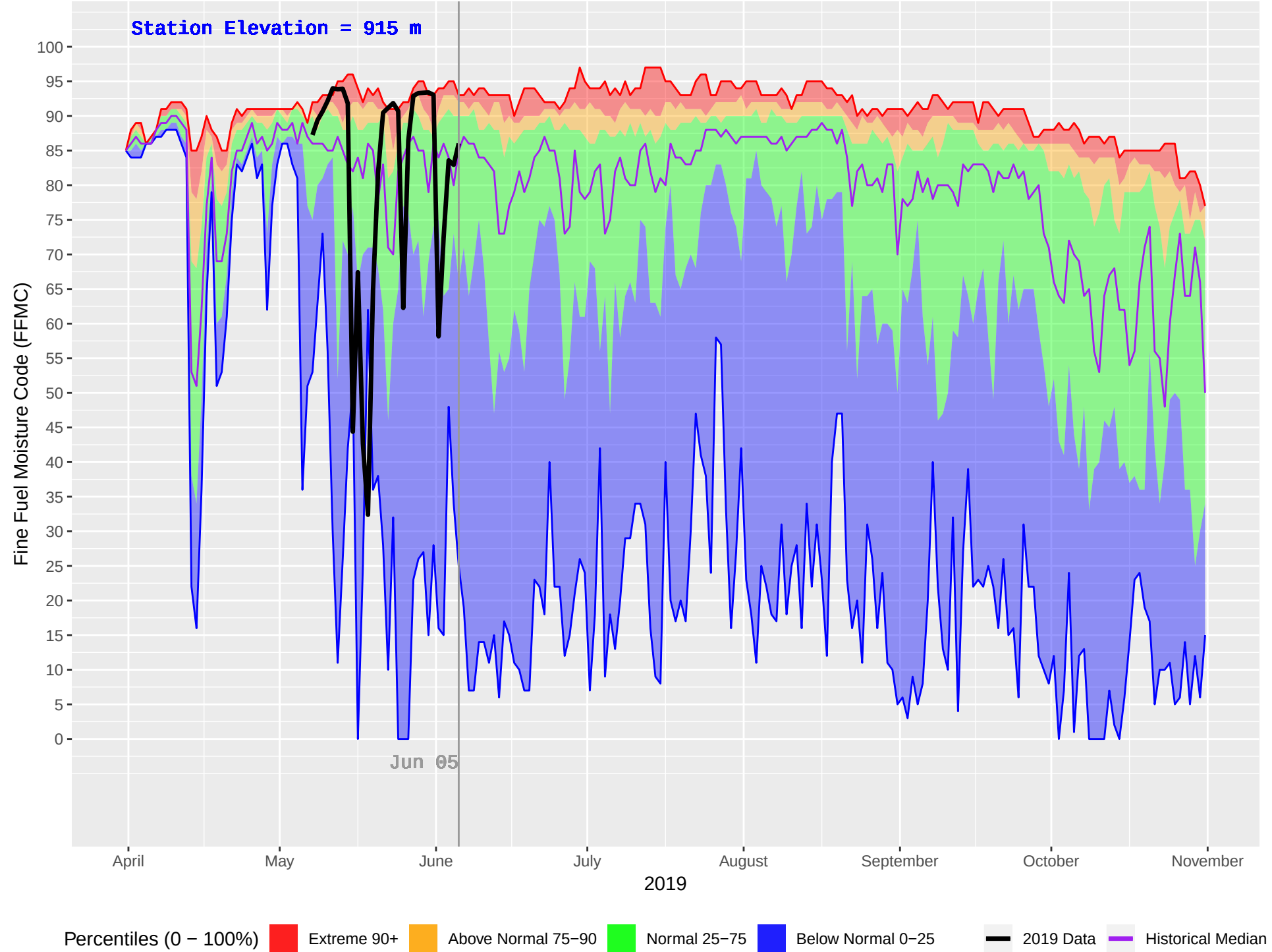
LEO CREEK (171) : Historical (1989–2018) and Current (2019) Daily Fine Fuel Moisture Code (FFMC)
