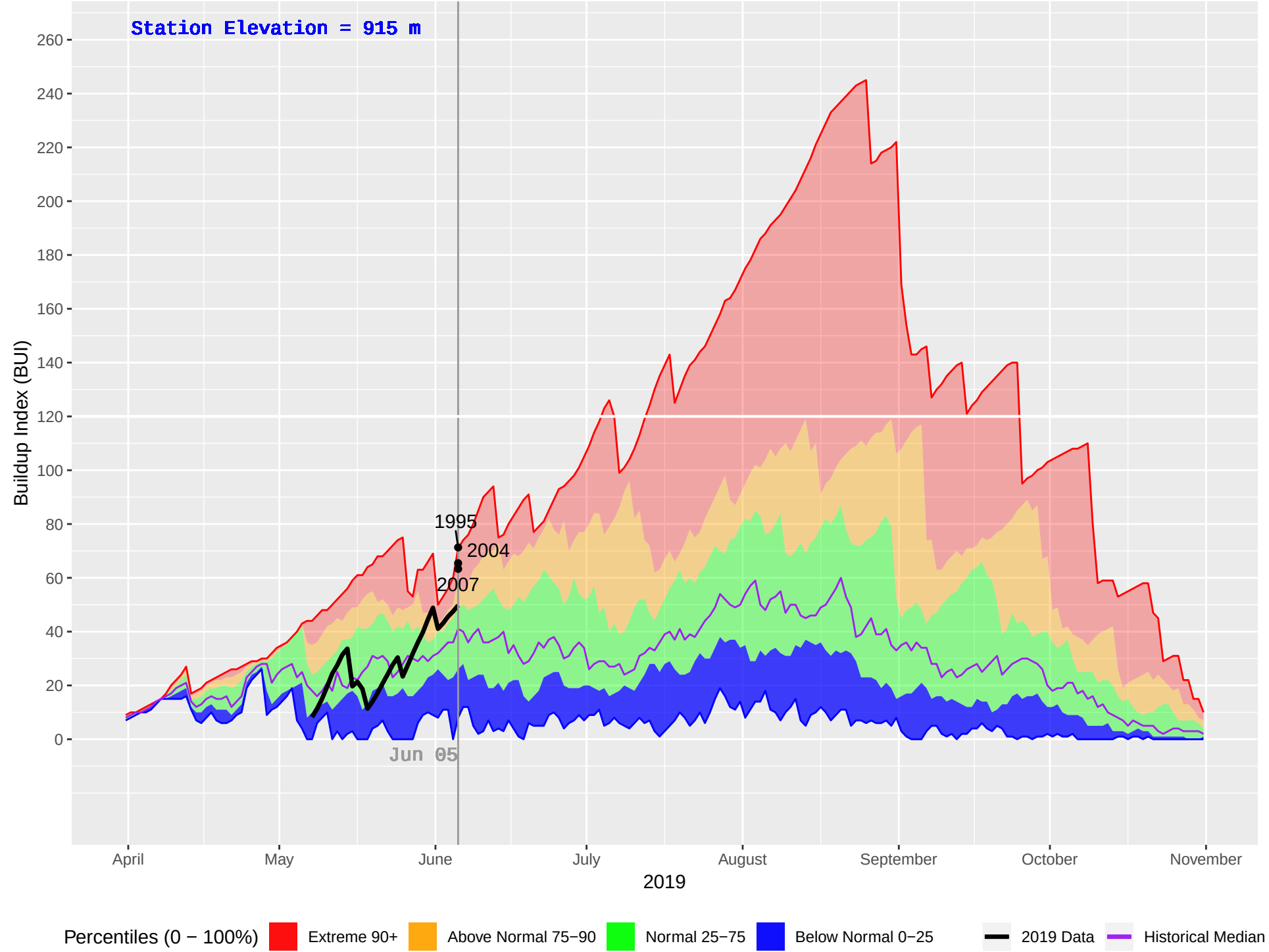
LEO CREEK (171) : Historical (1989–2018), Current (2019) Daily Buildup Index (BUI)
