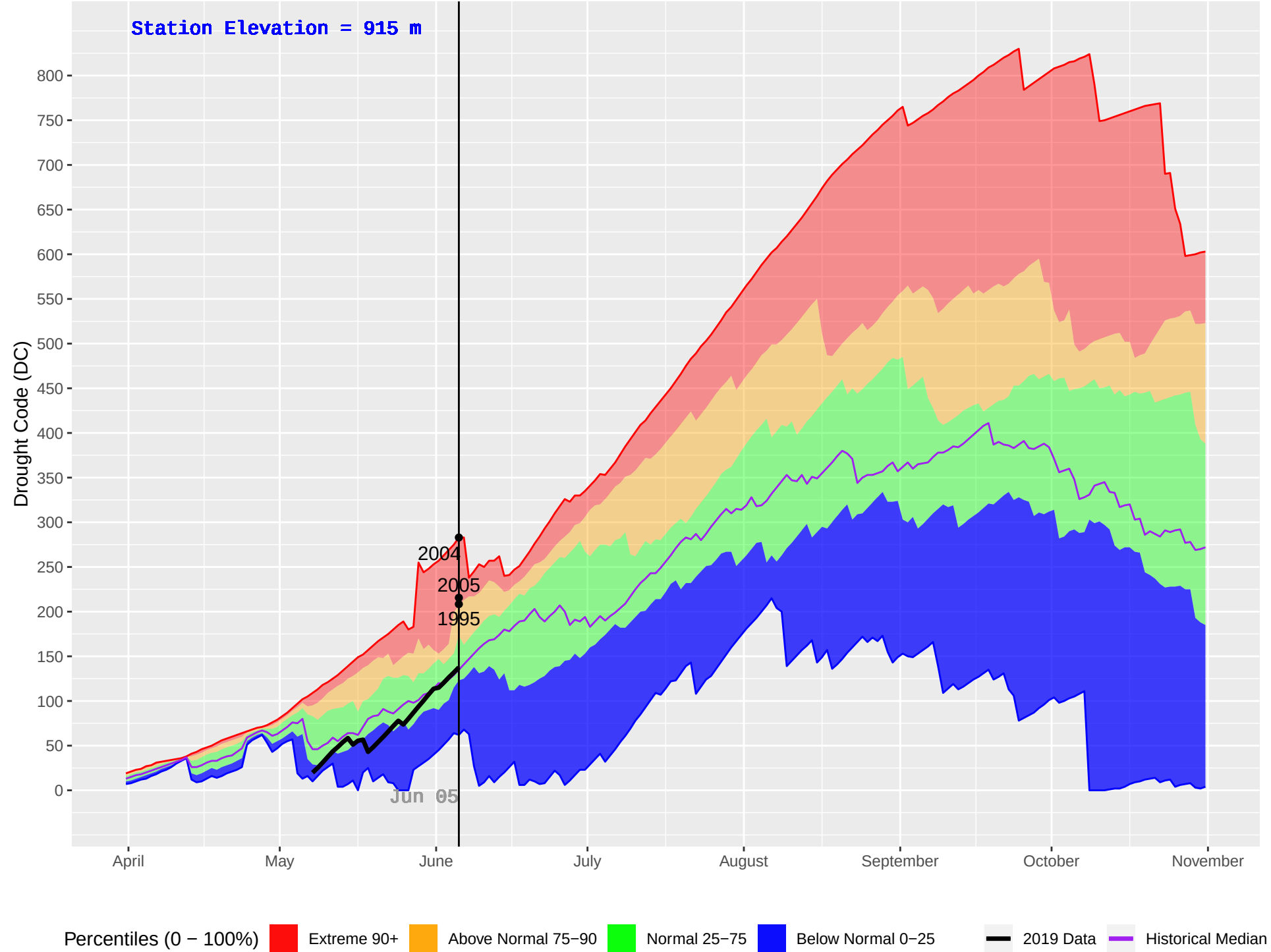
LEO CREEK (171) : Historical (1989–2018) and Current (2019) Daily Drought Code (DC)
