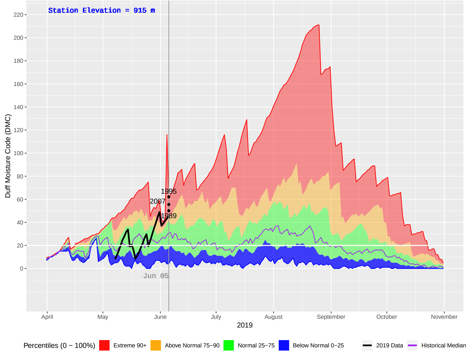
LEO CREEK (171) : Historical (1989–2018), Current (2019) Daily Duff Moisture Code (DMC)
