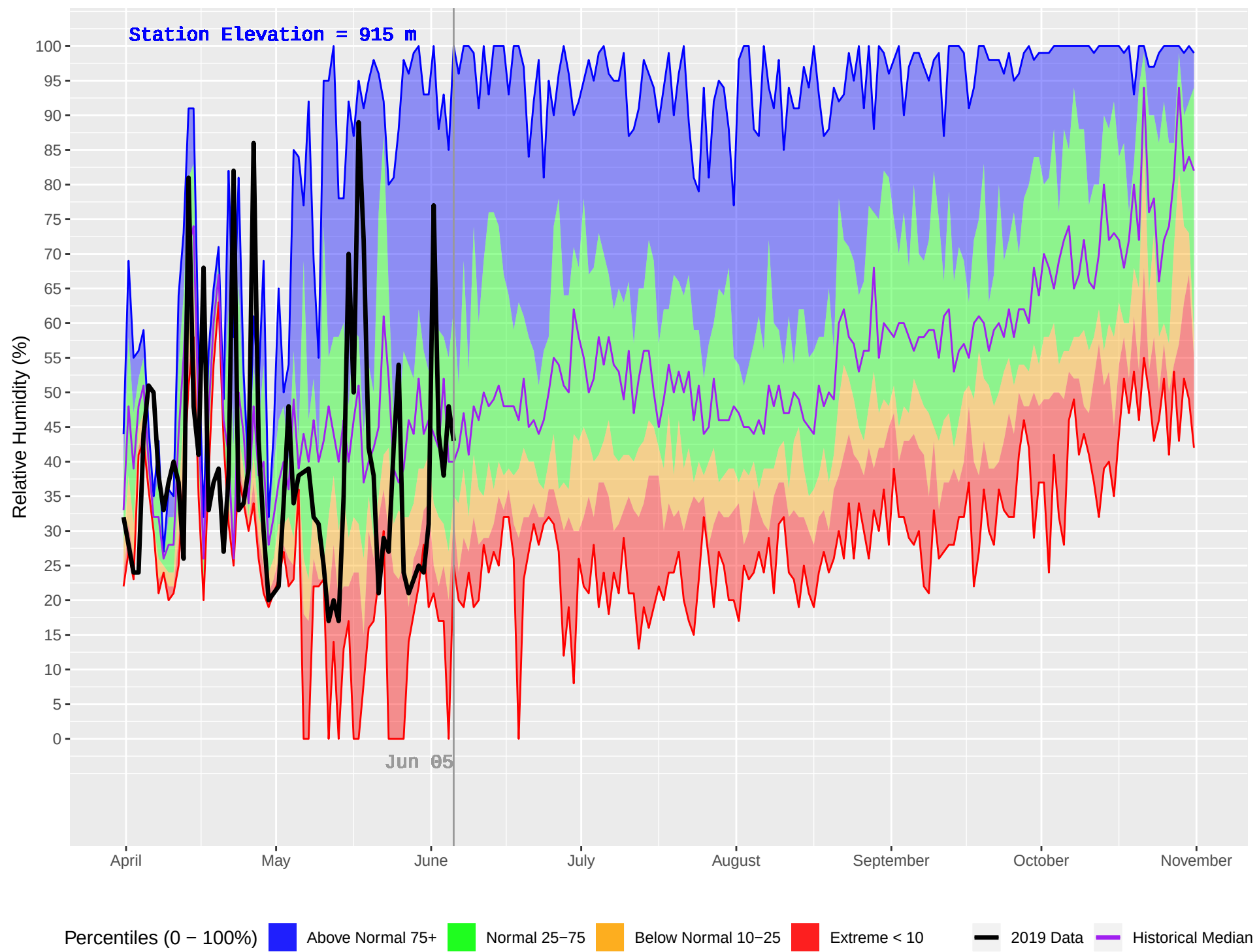
LEO CREEK (171) : Historical (1989–2018) and Current (2019) Daily Relative Humidity
