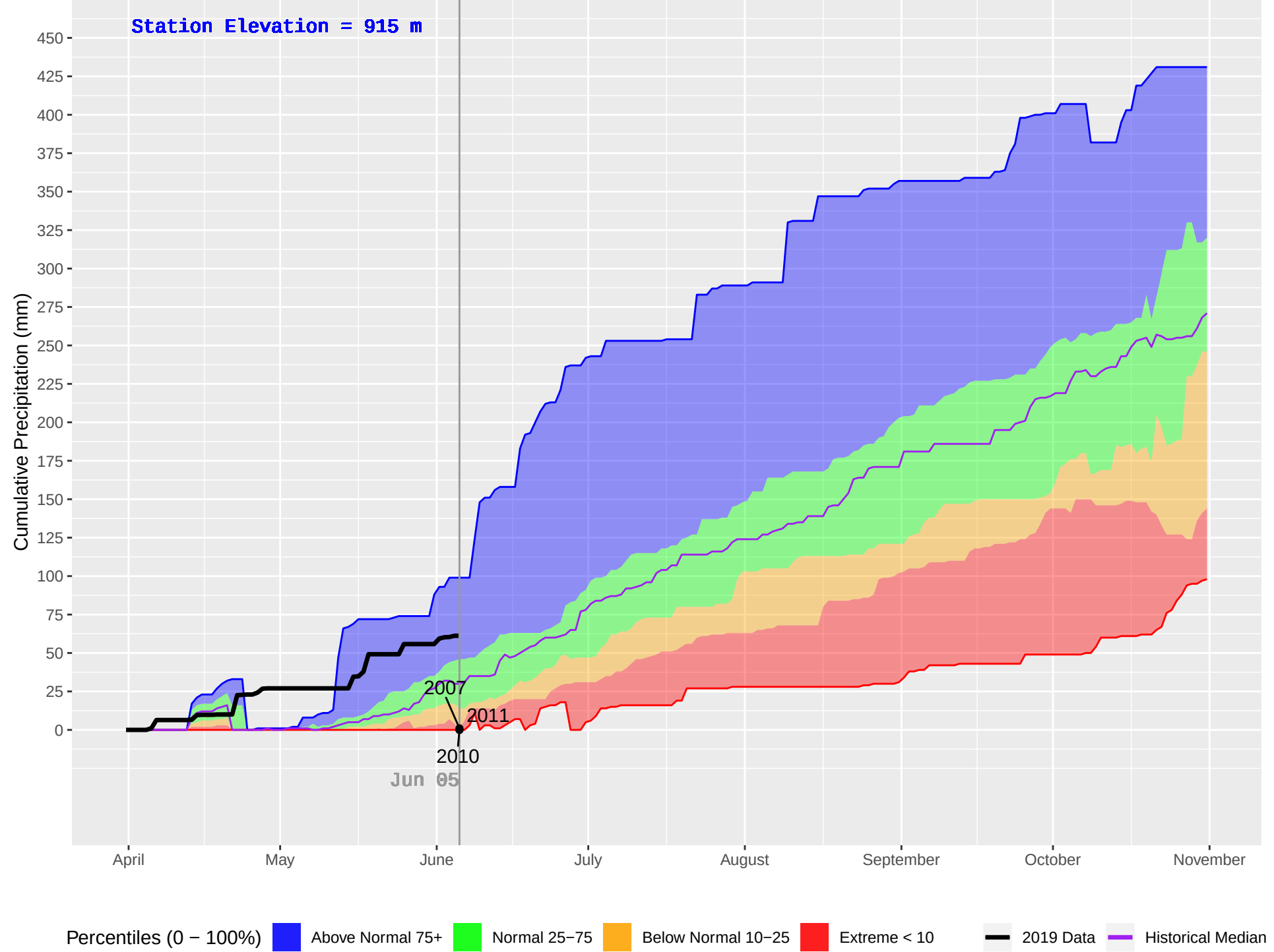
LEO CREEK (171) : Historical (1989–2018), Current (2019) Daily Cumulative Precipitation
